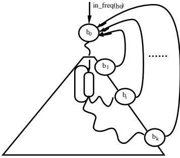
Figure 2. A two-head nested loop structure.
