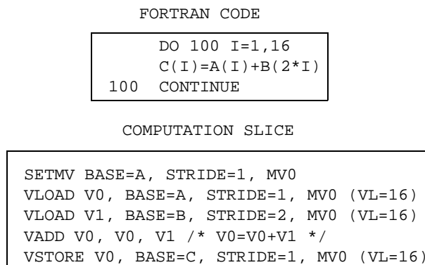
FIGURE 3. A SETMV instruction creates a mapping (stored in the mapping vector MV0) at the beginning of a computation slice. Memory instructions of the computation slice adhere to the mapping vector MV0.
