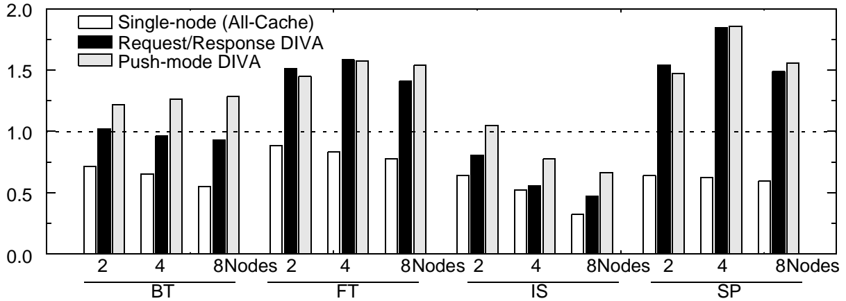
FIGURE 13. Relative performance of the DIVA systems and the single-node all-cache system normalized to the performance of the hypothetical case when applications would fit entirely in a single node.
