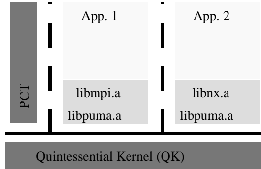
Figure 5: Puma Node Configuration: The Puma operating system on each node in the machine consists of the quintessential kernel (QK), a process control thread (PCT), and libraries linked with the applications running on the node. Only the QK runs in privileged mode. The QK, PCT, and each application run in separate address spaces. The solid, horizontal line separates user mode from supervisor (privileged) mode, and the dashed, vertical lines separate address spaces.
