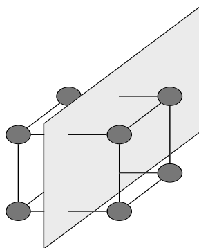
Figure 4: Bisection bandwidth: The nodes in a system are divided into two equal sized sets by an imaginary plane. The sum of the bandwidth of the communication links crossing the plane is the bisection bandwidth. The plane is placed so that the number of links crossing it is minimal and the number of nodes on each side is equal.
