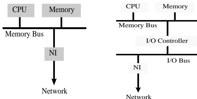
Figure 2: Network interface (NI) integration: On modern MP systems the network interface is either integrated into the CPU or is tightly coupled with the memory and CPU on a node, as shown on the left. Most workstations have an I/O controller, and the network interface is another device on the I/O bus. Often, this is a relatively low speed bus designed for high latency devices, such as disk, modems, and printers.
