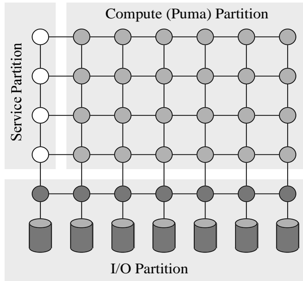
Figure 6: System Partitioning: A full-featured operating system is needed in the service partition to allow users to logon and to start parallel applications. In the case of the Intel Paragon, the Paragon OS, a variant of OSF 1/AD, authenticates users and provides full distributed Unix services. The Puma QK and PCT run on each node in the compute partition. The operating system running in the I/O partition could be Puma or another operating system with the appropriate driver for the I/O device and the capability to exchange messages with Puma.
