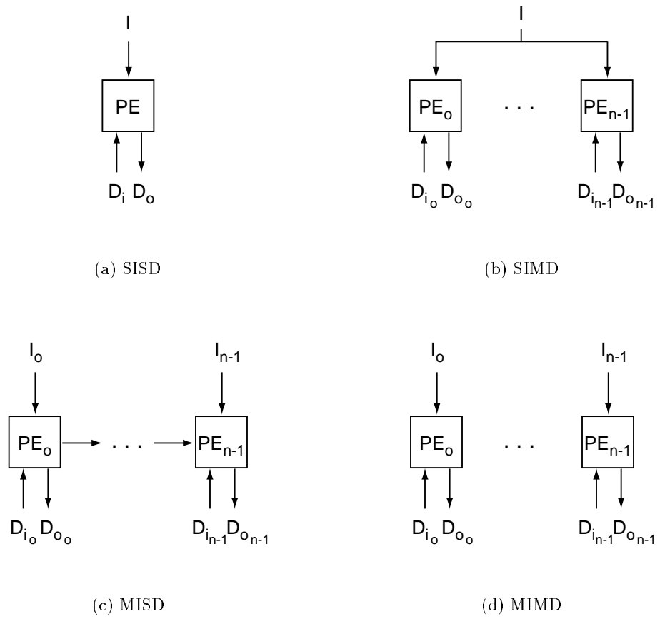
Figure 1: The Stream Model
