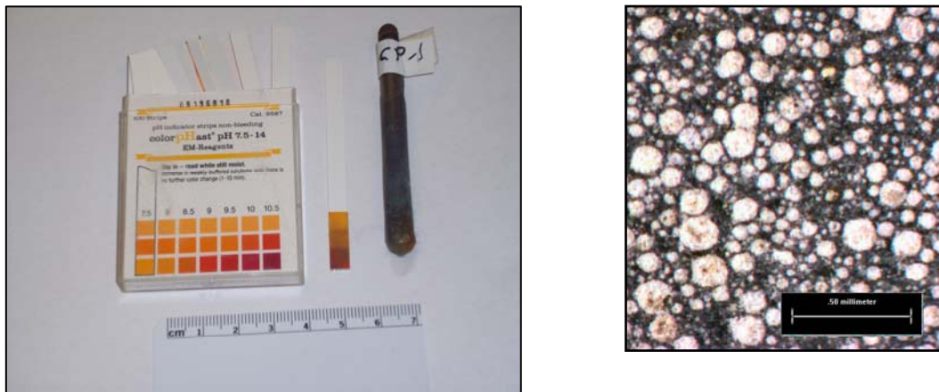
Figure 3. Enamelled test rod with portland cement embedded in the glass (left) and polished section of side of rod after exposure (right). The moist pH test strip applied to the surface showed the pH of the abraded surface was approximately 10.5.
