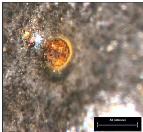
Figure 6. Optical photomicrograph of the edge of a hole drilled in the enamel to expose underlying metal. Rod sample was exposed to 3.5 percent NaCl solution for 40 days to produce corrosion. The enamel does not debond or allow capillary transfer of salt solutions.
