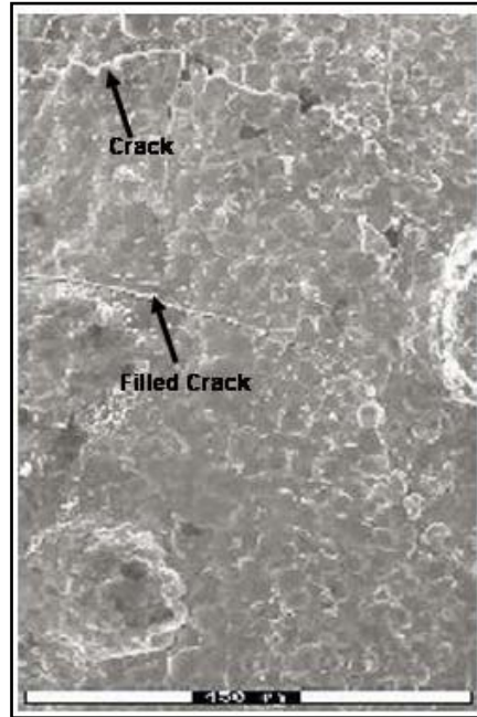
Figure 7. Surface of enameled metal wire bent to produce fractures and partly wetted to produce examples of open and filled fractures. The reacted cement on the surface produces the irregular surface texture.
