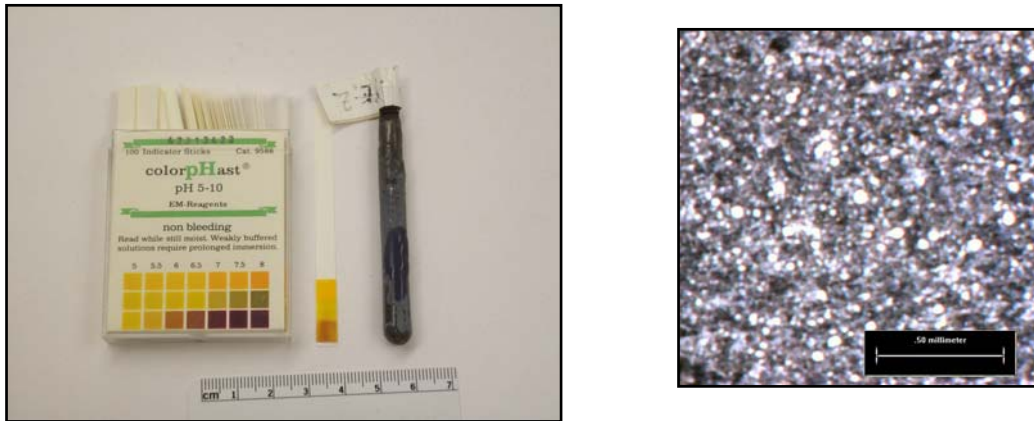
Figure 2. Enamelled test rod (left) and polished section of side of rod after exposure (right). The moist pH test strip applied to the surface showed the pH of the abraded surface to be approximately 6.5.
