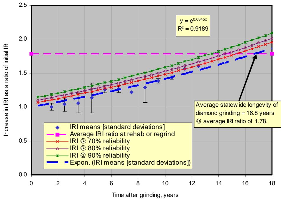
Figure 2. Reliability levels for the expected survivability of California diamond-grinding projects (2).
