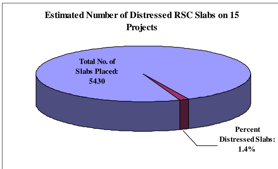
Figure 9. Percent distressed slabs on surveyed RSC projects (13).
