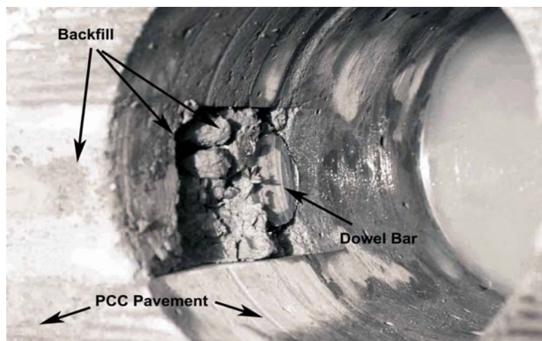
Figure 7. A poorly performing dowel bar retrofit on I-5 in Orange County (10).
