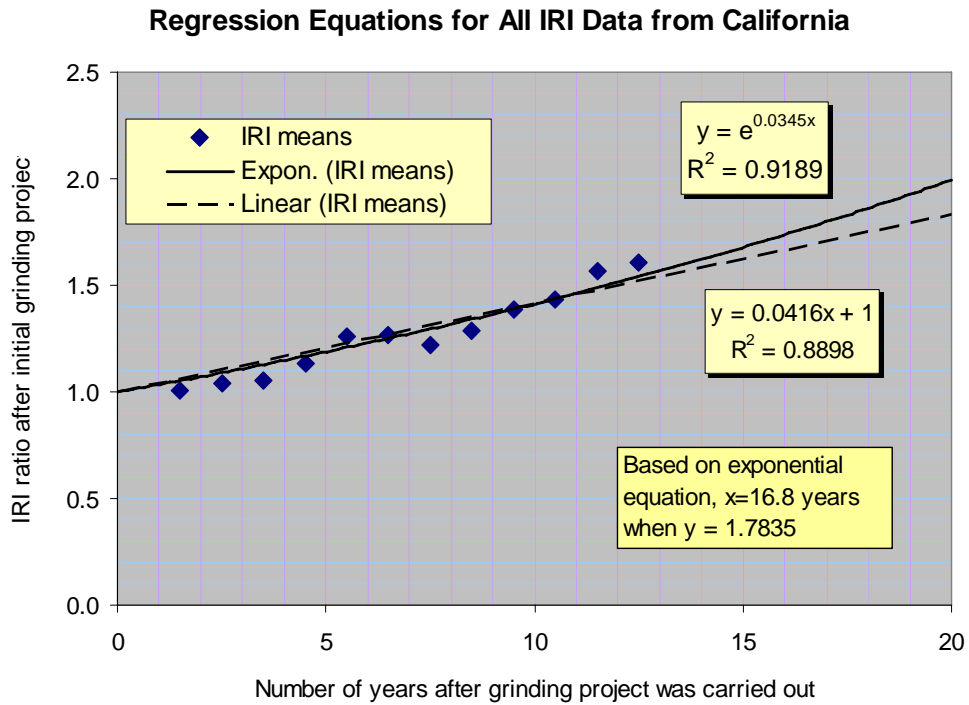
Figure 1. Change in the ratio of IRI over time as a function of the initial IRI after grinding (2).
